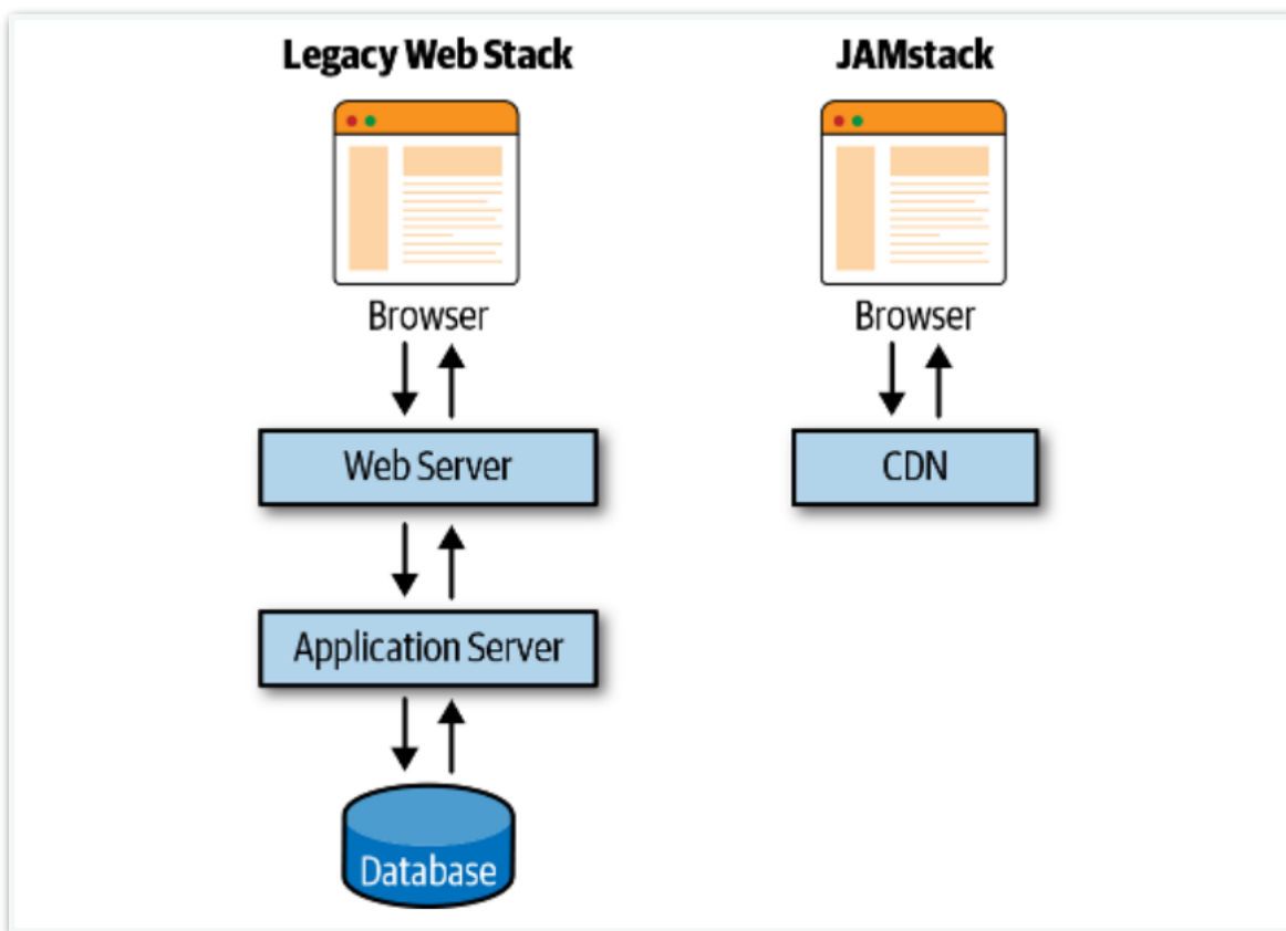
Figure 3-1. Legacy web stack versus Jamstack
